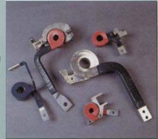
Blowout Coils with Supports and Insulation
